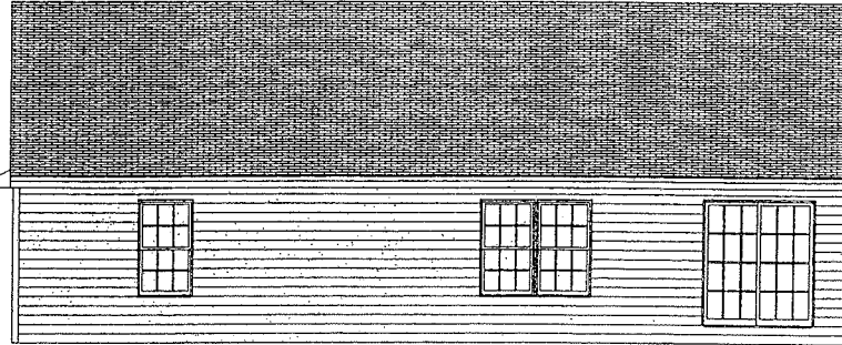
REAR ELEVATION
